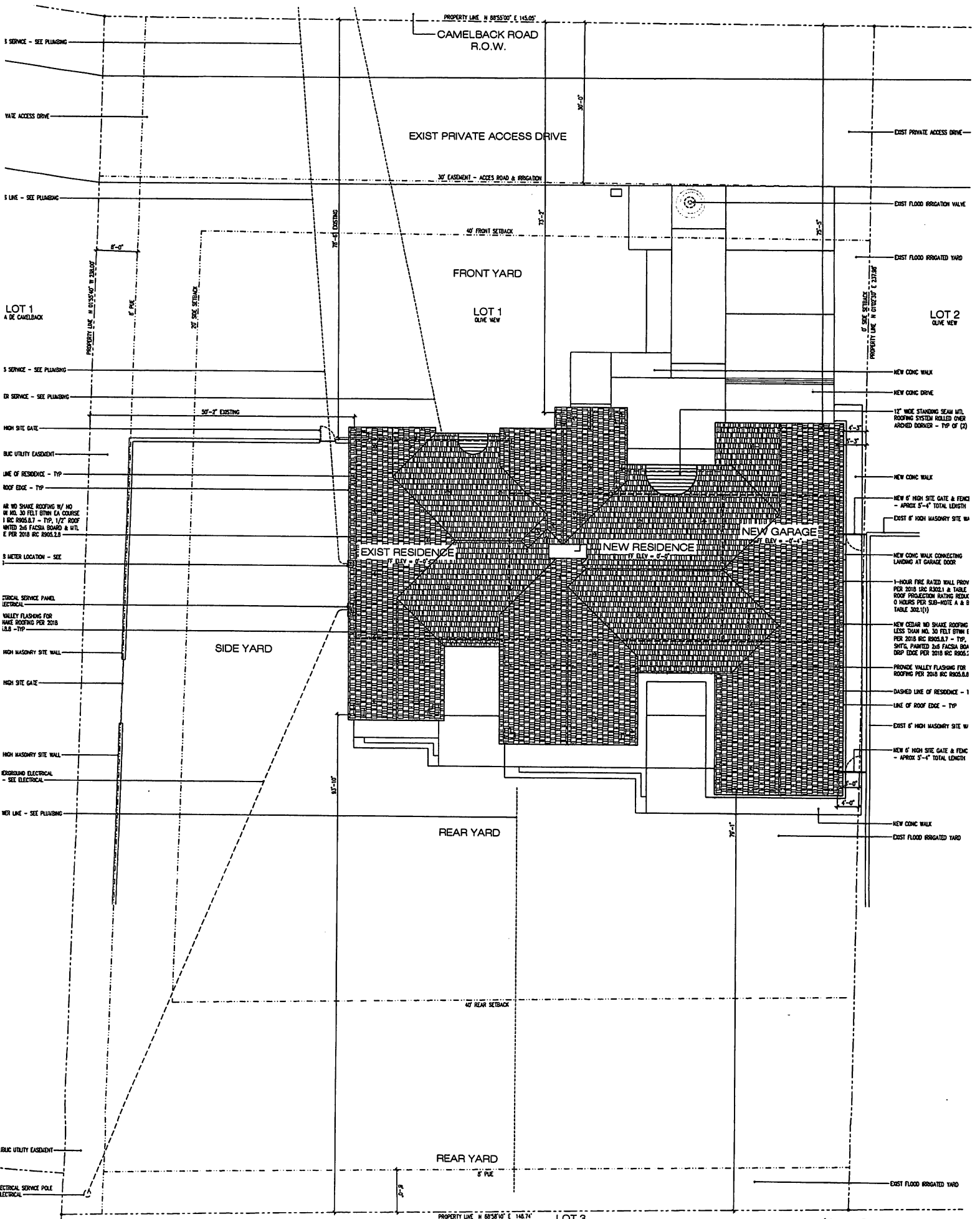
site & roof plan
